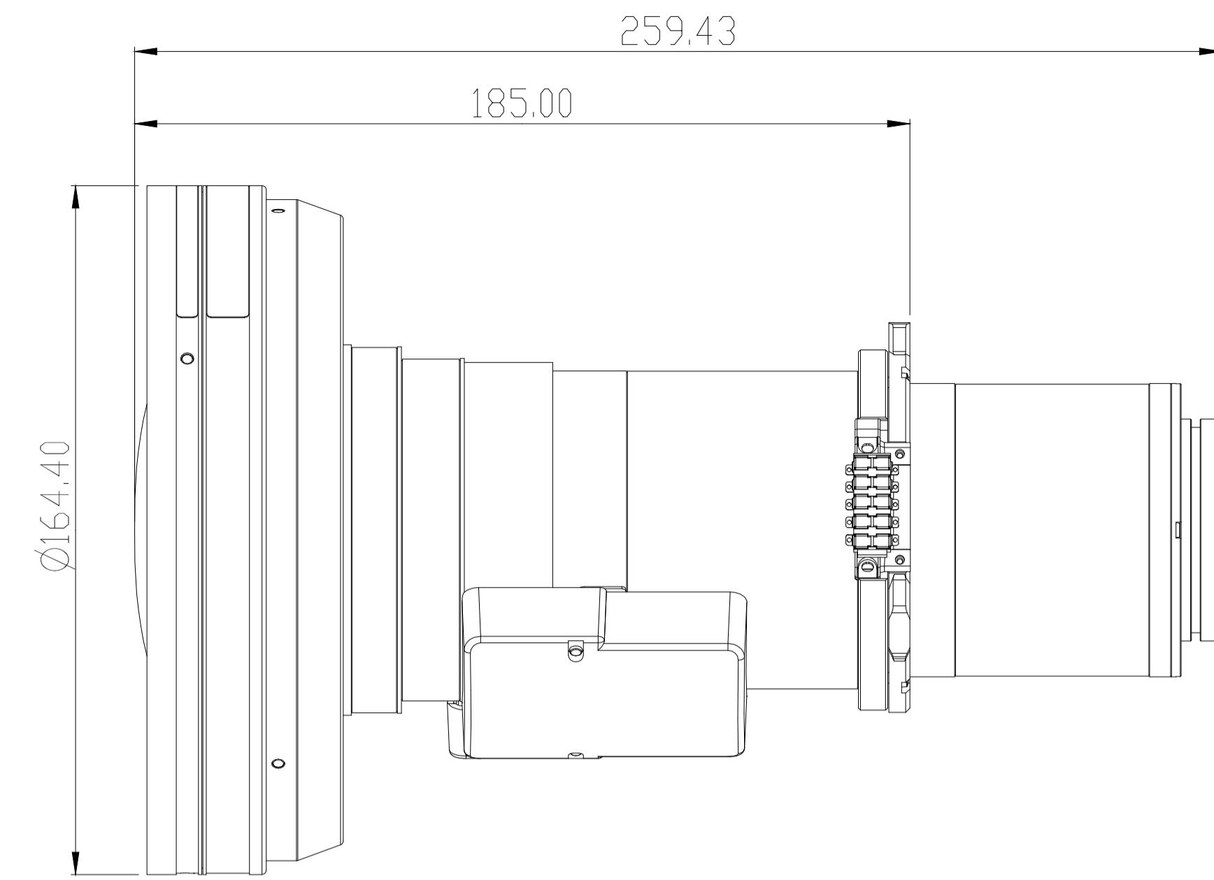
TR 0.84~1.02 WIDE ZOOM (BX-CTA18)
