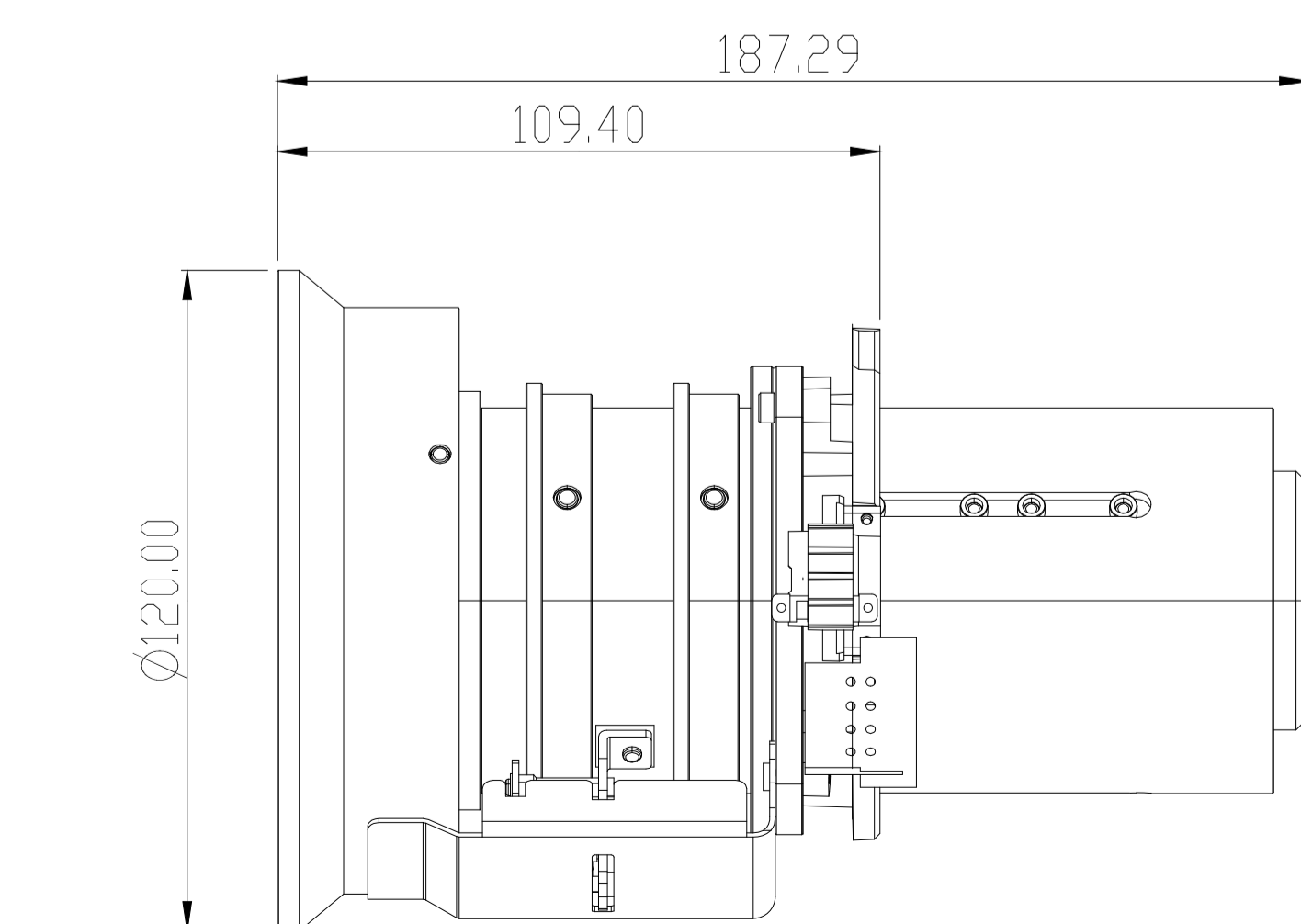
TR 1.02~1.36 WIDE ZOOM (BX-CTA19)
