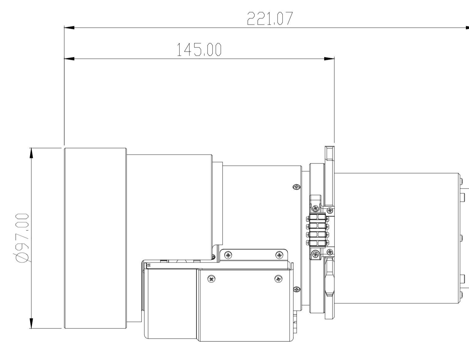
TR 1.50~2.00 STANDARD ZOOM (BX-CTA21)
