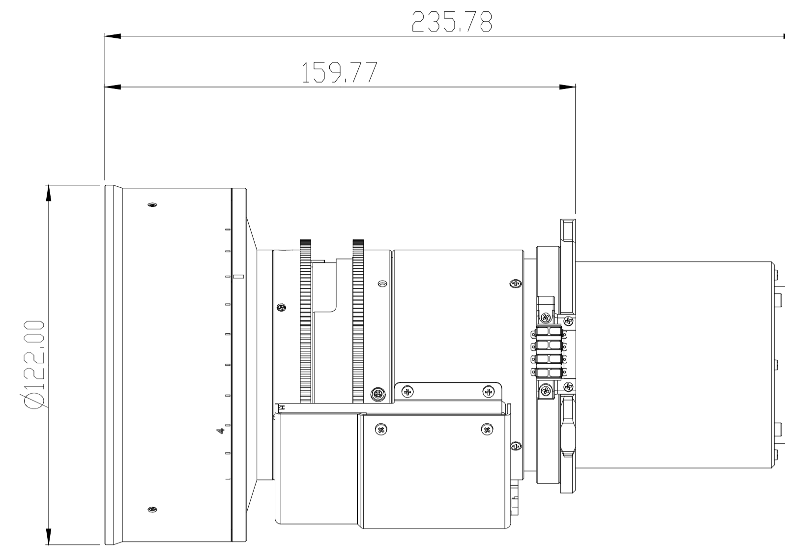
TR 1.20~1.50 WIDE ZOOM (BX-CTA20)
