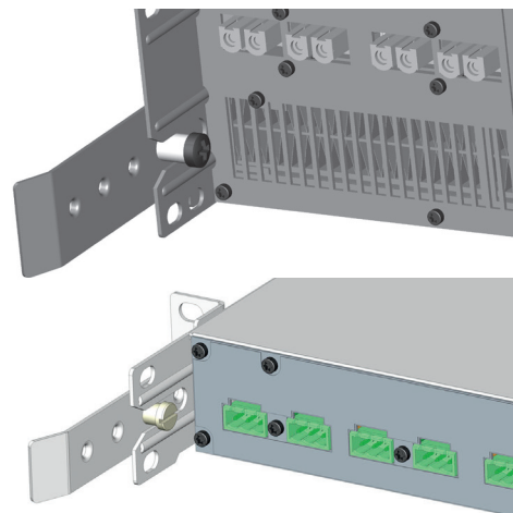
Rear support bracket mounted for removable installation and bracket pointing towards back
