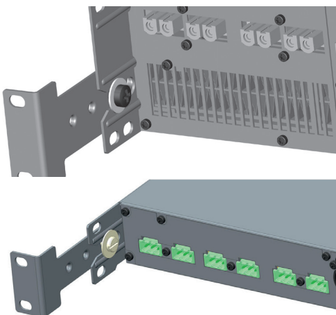
Rear support bracket with mounting hardware
