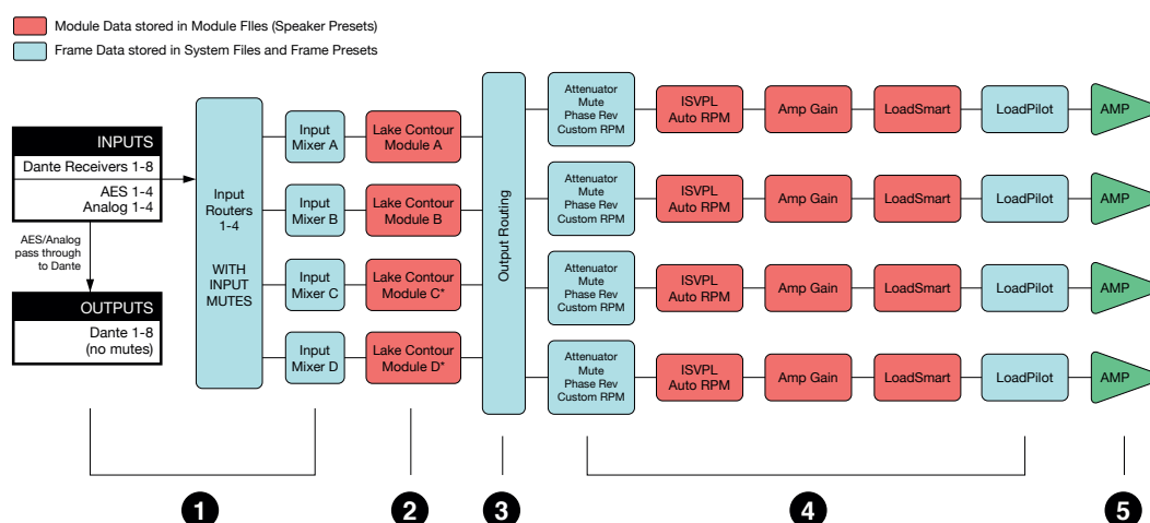
Figure 12.1: K&F D Series Lake Signal Flow Diagram
