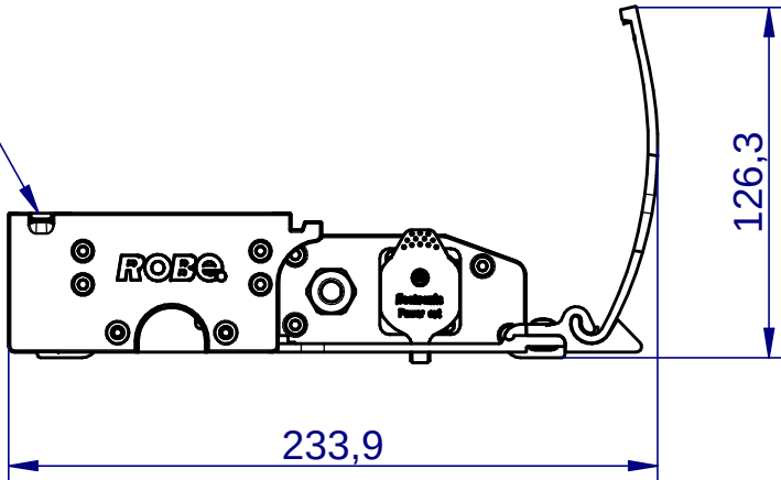
Cover in open position
