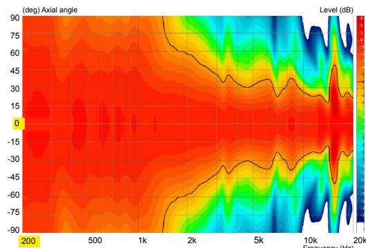
iBeam Waveguide Linienstrahler - Directivity - horizontal
