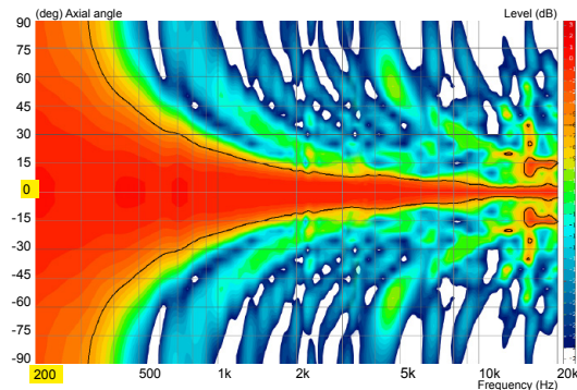
iBeam Waveguide Linienstrahler - Directivity - vertical
